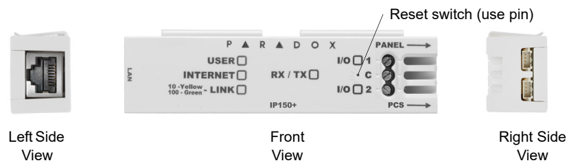
Figure 2 - IP150+ Overview
